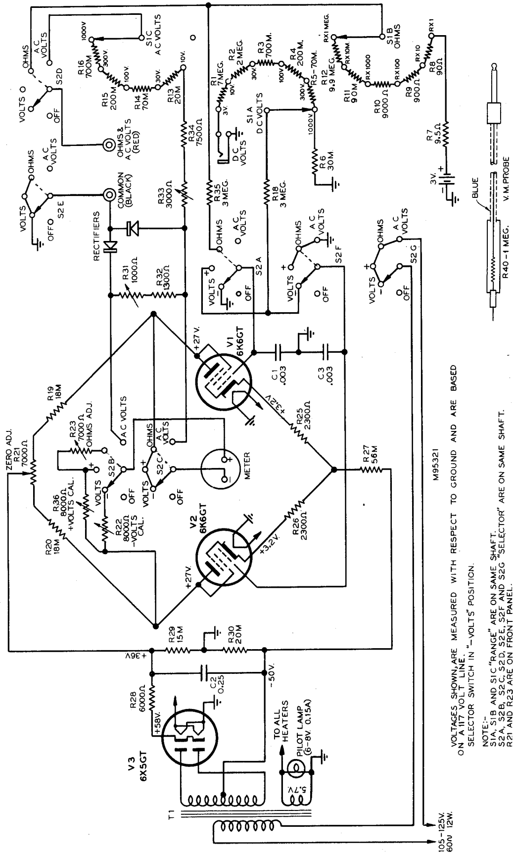
Figure 1—Schematic Circuit Diagram, Type No. 165-A, Code 943
